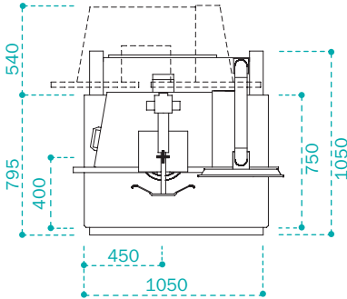
T14 | Vista superior
